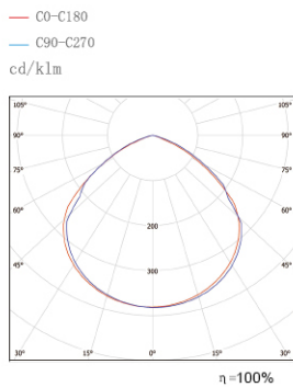
配光曲线/Light Distribution Curve:
